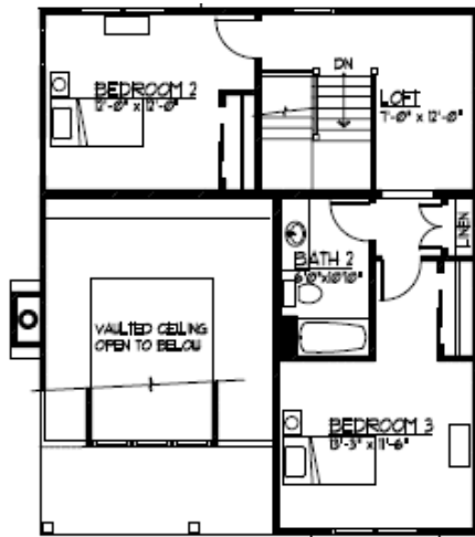
SECOND FLOOR ELEV a
