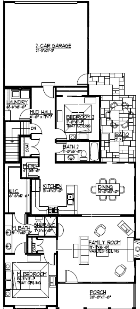
FIRST FLOOR ELEV a - LOT #1, 14, 28
