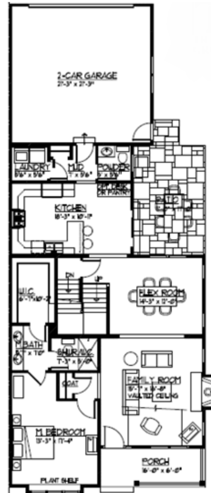
FIRST FLOOR ELEV a - LOT #6, 30
