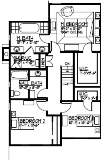
SECOND FLOOR ELEV a - LOT #4, 21, 31
